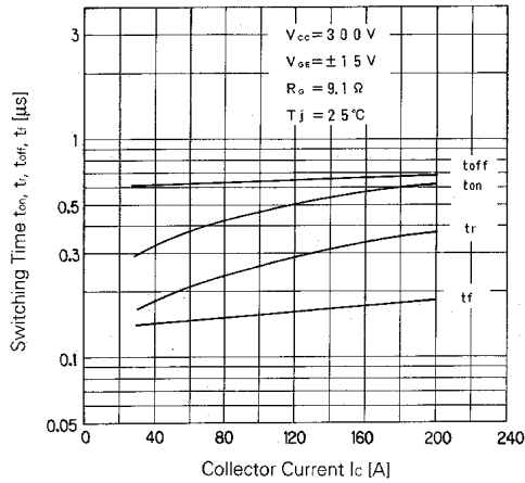
Switching Time
