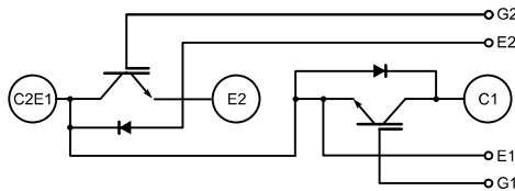
Outline Drawing and Circuit Diagram
